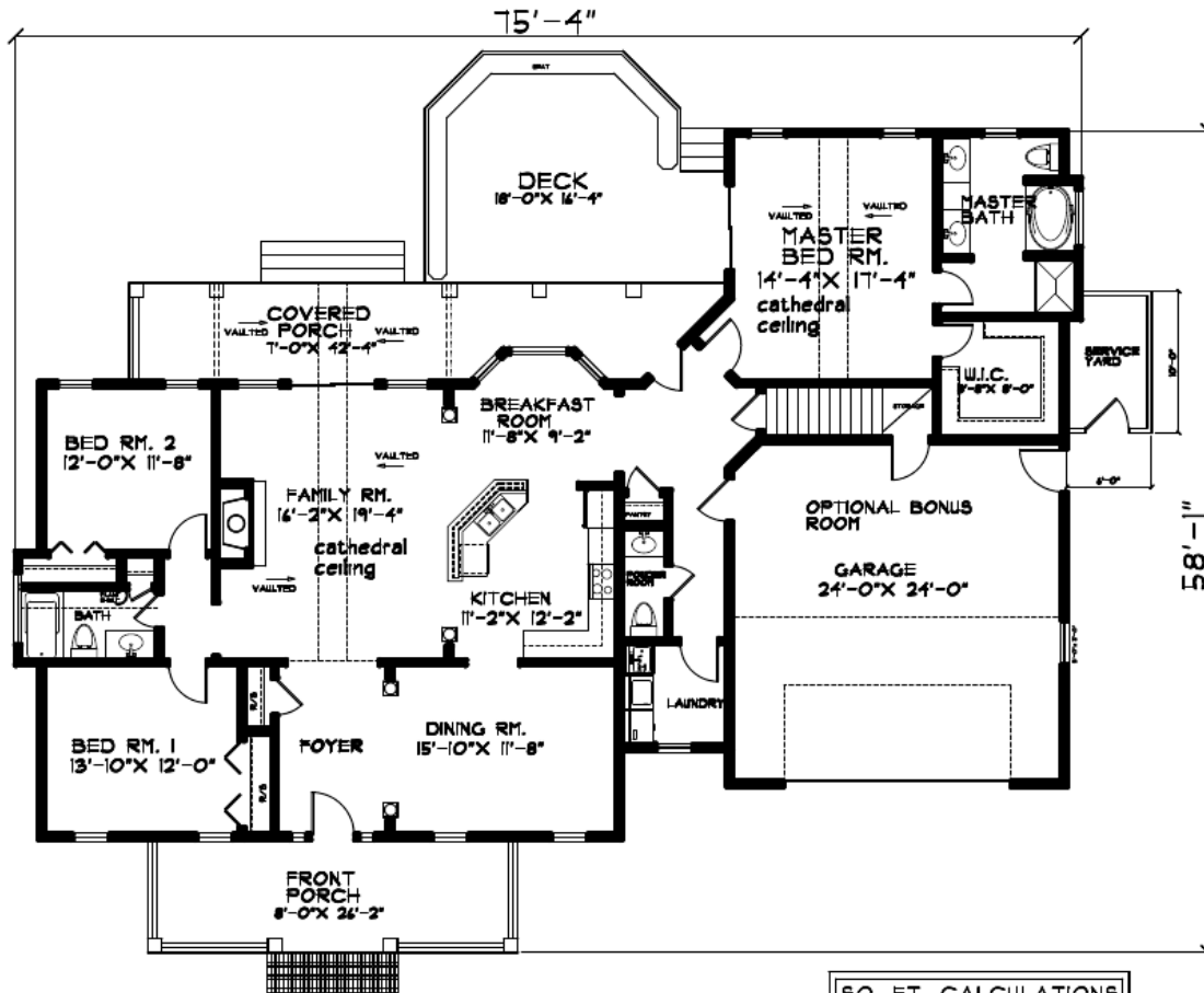
FLOOR PLAN MODEL WHITNEY
